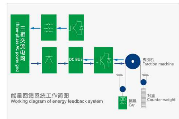
能量再生回馈技术 Energy regeneration and feedback technology
